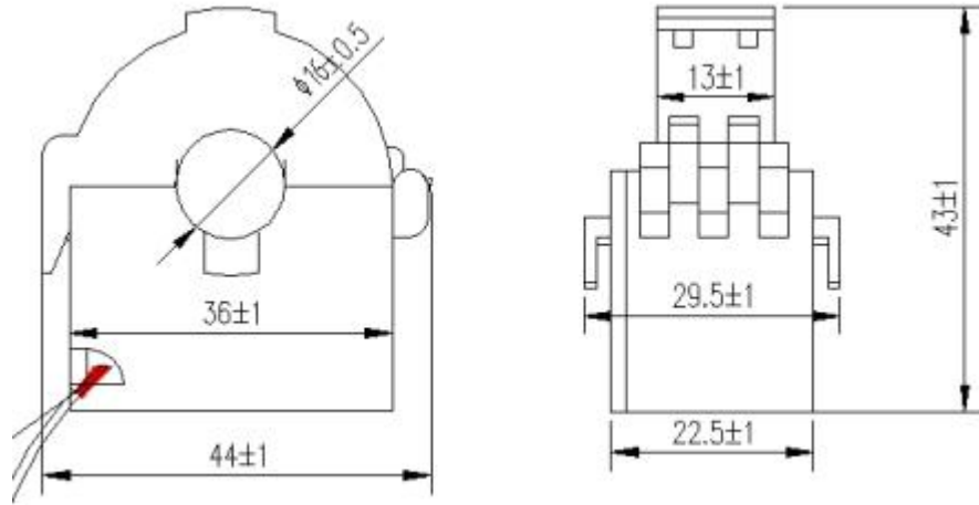
Figure 3 Dimension of current transformer
